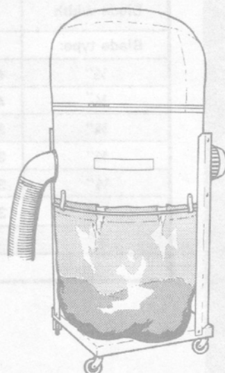
'CYCLAIR 55' Dust Extractor Inlet diameter: 4¼" Suction rate: 565 ft³/min Collection capacity: 5 ft³
