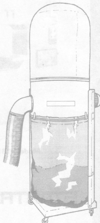
'CYCLAIR 75' Dust Extractor Inlet diameter: 6¼" Suction rate: 1045 ft³/min Collection capacity: 9 ft³
